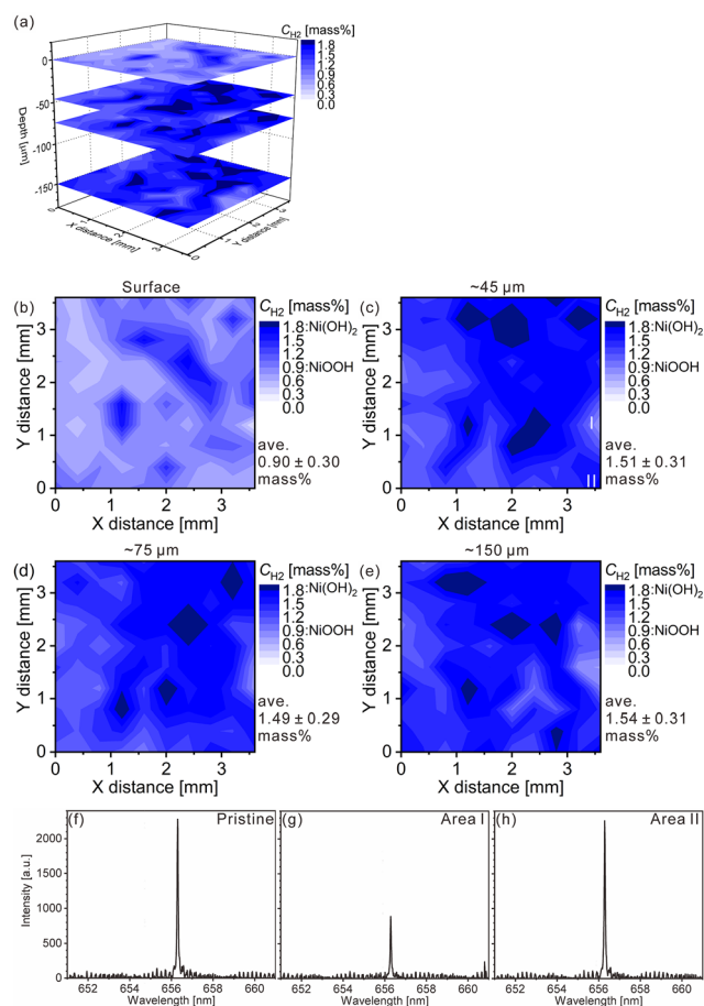
Fig. 3 LIBS maps of the hydrogen concentrations (mass%) in the model cathode after the fifth charging for (a) 3D illustration and 2D illustrations of the (b) first layer, (c) third layer (~45 \mu\text{m} in depth), (d) fifth layer (~75 \mu\text{m} in depth), and (e) tenth layer (~150 \mu\text{m} in depth). LIBS spectra of (f) the pristine cathode of the third layer and the model cathode after the fifth charging for areas (g) I and (h) II in Fig. 3(c).
