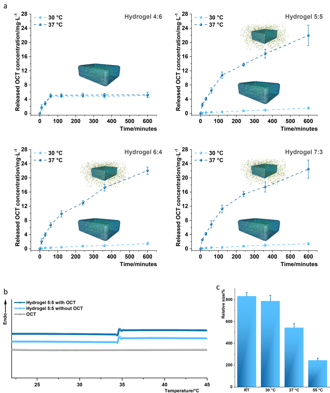
Fig. 2 Characterization of the fabricated hydrogels. (a) Analysis of thermo-regulated OCT release from OCT-loaded hydrogels 4 : 6, 5 : 5, 6 : 4, and 7 : 3 samples through a UV-visible spectrophotometer as reported. 4 Cumulative OCT in vitro release from hydrogels 4 : 6, 5 : 5, 6 : 4, and 7 : 3 samples loaded with OCT was assessed at 30 °C (light blue dashed lines) and 37 °C (dark blue dashed lines). The total OCT amount loaded in hydrogels 4 : 6, 5 : 5, 6 : 4, and 7 : 3 was determined to be 7.8 \pm 0.7 mg L -1 , 28.9 \pm 1.1 mg L -1 , 27.7 \pm 1.9 mg L -1 and 28.4 \pm 0.9 mg L -1 , respectively, after a thorough OCT release from the corresponding hydrogel in PBS at 50 °C for 3 days. The in vitro release analysis was conducted three times with three replicates, and every replicate was measured three times. One set of measurements has been displayed together with standard deviations (error bars) derived from 9 data. (b) The sol–gel transformation of the designed hydrogel was herein analyzed by differential scanning calorimetry (DSC) in PBS buffer (pH 7.4) to characterize the LCST in a consecutive heating process. The identified LCSTs were respectively 34.3–35.3 °C and 34.2–35.2 °C for hydrogel 5 : 5 with and without loading of OCT. The LCST was measured five times for every sample, and one data set was displayed. (c) The relative size of hydrogel 5 : 5 after completely swelling. The sizes of hydrogel 5 : 5 were respectively measured three times by a graduated cylinder at room temperature (RT) after swelling for 5 days in deionized water and at 30 °C, 37 °C, and 55 °C after incubation for 4 hours. All the measured sizes were aligned to the original mold size (0.3 mL) to fabricate the hydrogel.
