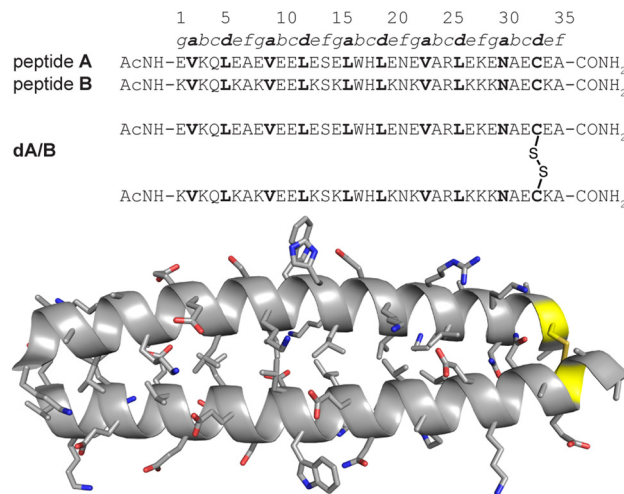
Fig. 1 Sequences of acidic monomer A; basic monomer B; and disulfide-bound heterodimer dA/B. Also shown is the ribbon diagram of dA/B (PDB ID: 1KD9) with side chains shown as sticks and Cys33–Cys33' disulfide highlighted in yellow.
