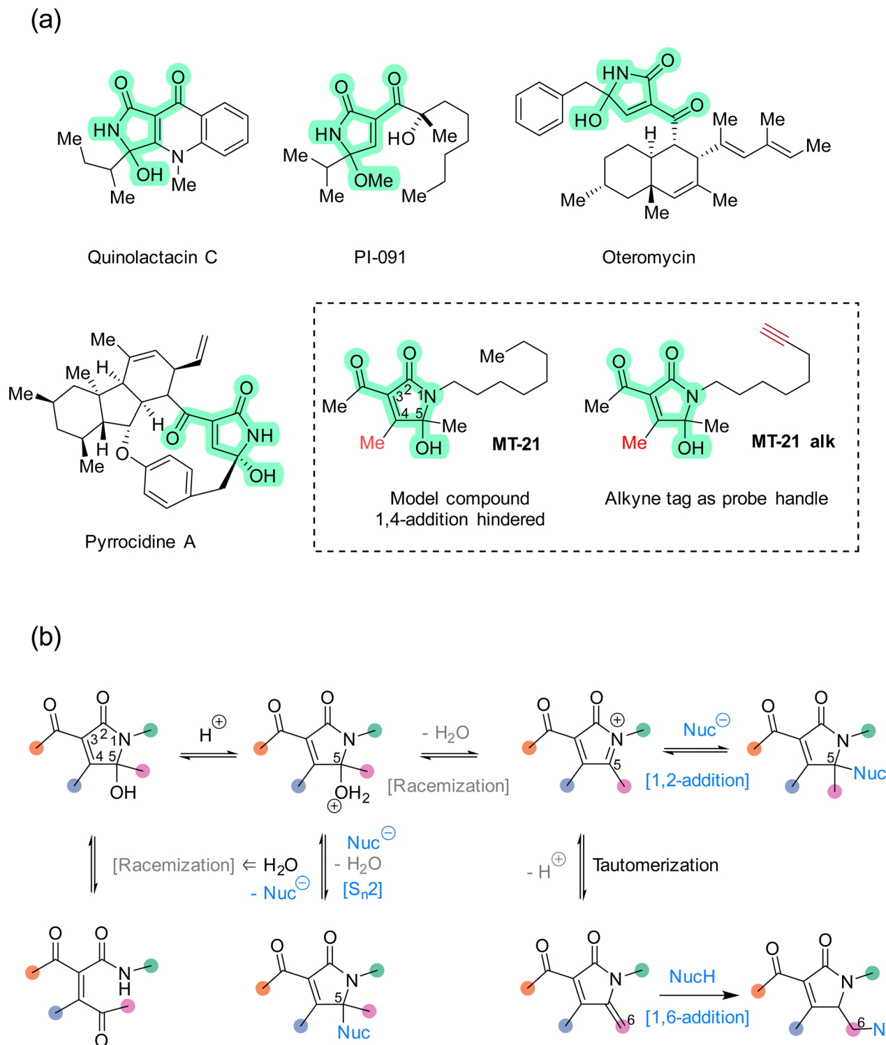
Fig. 1 (a) Examples of natural products that contain the AHPO-scaffold and structure of the synthetic compound MT-21 and its associated alkyne-tagged version MT-21 alk . (b) Within the AHPO-scaffold, racemization of the N -acyl hemiaminal stereocenter at C5 may occur either via N -acyl hemiaminal reversal or through iminium ion formation, the latter can further tautomerize to form an extended Michael acceptor. With an AHPO-scaffold sterically blocked at C4, nucleophiles may react at C6 (via 1,6-addition) or at C5 through either 1,2-addition to the iminium ion or by direct substitution. The latter would not compromise stereochemical integrity, unless the nucleophile is water.
