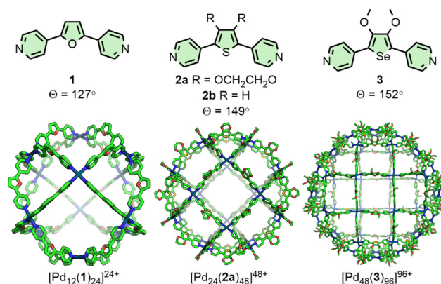
Fig. 1 Dipyrpyridyl ligands 1 , 2 , and 3 self-assemble with Pd(II) ions to form Pd 12 L 24 , Pd 24 L 48 and Pd 48 L 96 assemblies (SCXRD structures), respectively, with the angle between coordinating groups determining the nuclearity of the thermodynamically favoured product.
