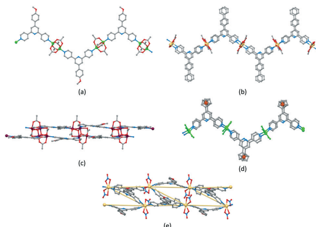
Fig. 9 (a) Part of the zigzag chain in [Zn_2(OAc)_4(4'-(4-MeOC_6H_4)-4,2':6',4''-tpy)]_n (CSD refcode SOXSEF). Parts of the double stranded zigzag chains in (b) [Cd_2(OAc)_4(4'-(4-PhC_6H_4)-4,2':6',4''-tpy)]_n (refcode RIGJEY), (c) [Cu_4(\mu_3-OH)_2(OAc)_6(4'-(4-MeOC_6H_4)-3,2':6',3''-tpy)_2]_n (refcode KUCHIC), and (d) [Zn_2Cl_2(1,1'-bis(4,2':6',4''-terpyridin-4'-yl)ferrocene)]_n (refcode UMUYUY). (e) Part of the ladder assembly in [Cd_2(4'-(4-MeOC_6H_4)-4,2':6',4''-tpy)_3(NO_3)_4]_n (refcode BUDZIL); the Cd...Cd vectors which define the ladder are highlighted.
