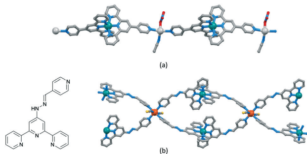
Fig. 8 (a) Part of the linear 1D-chain in [(Ru(pytpy)_2Ag(NCMe)(NO_3))_n][NO_3]_{2n} \cdot nH_2O \cdot nMeCN (CSD refcode WICSIL). (b) Structure of ligand 6 and part of the chain comprising interconnected loops in [(Fe(NCS)_2(Ru(6)_2)_2)_n][Fe_2(NCS)_6(OEt)_2(EtOH)_2]_n[NCS]_{2n} \cdot 4nEtOH \cdot nH_2O (CSD refcode TOPLIU).
