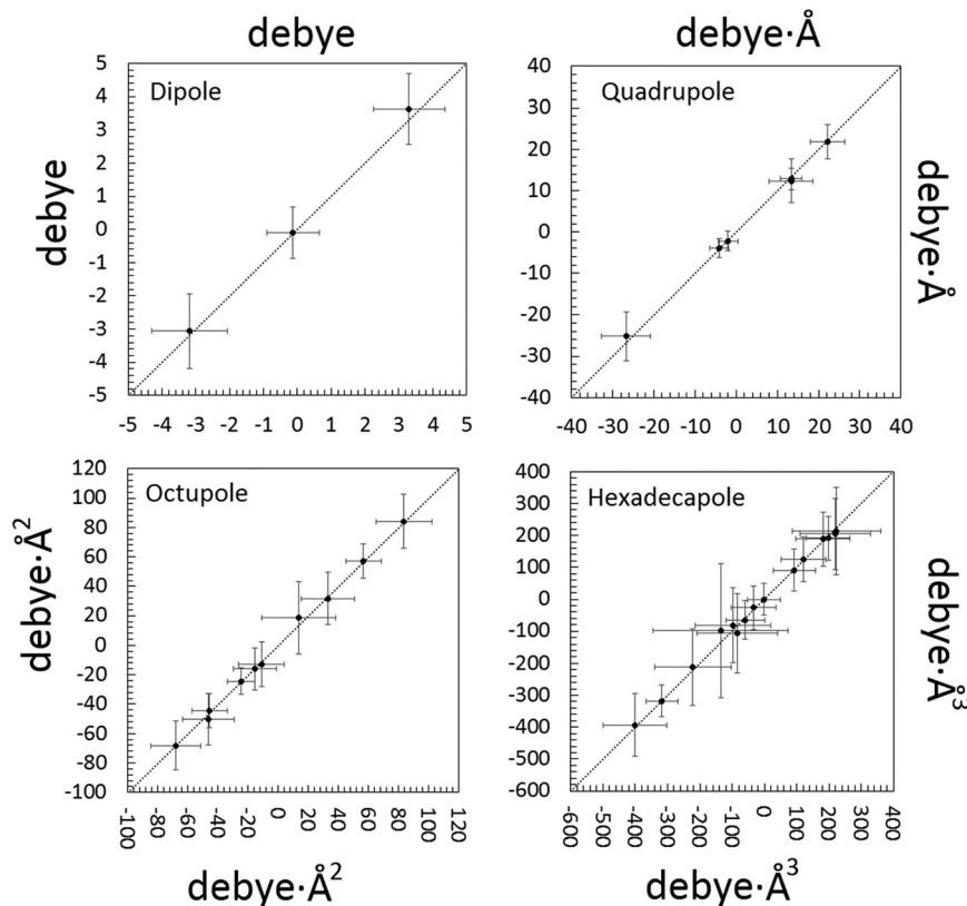
Fig. 5 Correlation between electrostatic unbridged moments of the NCLBA molecule extracted from the crystal estimated by multipolar and QTAIM traceless Cartesian moments of pseudoatoms ( x axis) vs. traceless Cartesian moments of QTAIM atoms ( y axis). Origin: molecular centre of mass; reference system: inertial frame. Data points are represented by their error bars, corresponding to the pooled standard deviation. The dashed 45 deg lines represent perfect agreement. See Table S7 ESI† for the corresponding numerical entries.
