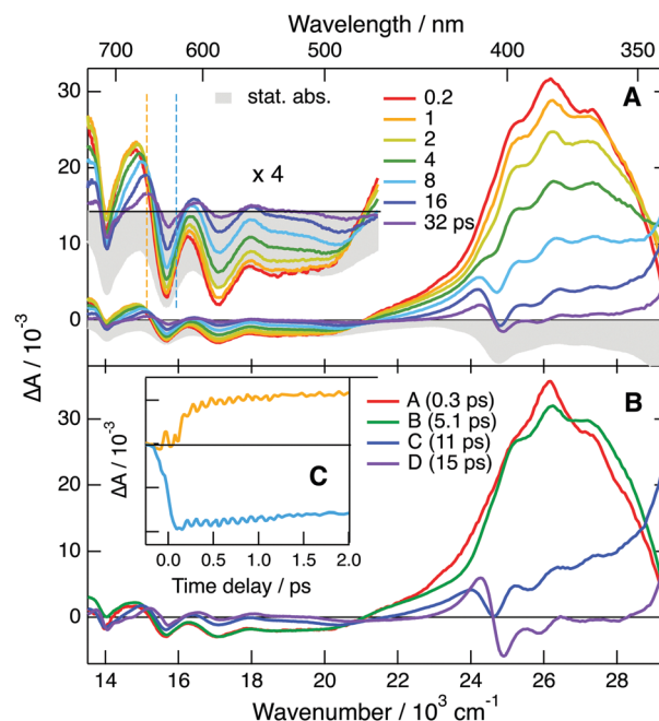
Fig. 7 (A) Transient absorption spectra measured various time delays after 710 nm excitation of TrCA •- generated upon continuous irradiation of a TrCA/TEA/TBADHP solution, and negative stationary absorption spectrum. (B) Evolution-associated difference absorption spectra and time constants obtained from a global analysis of the transient absorption data assuming four successive exponential steps, A \rightarrow \dots \rightarrow E , E being the ground state. (C) Time profiles of the transient absorption at the wavenumbers shown by the dashed lines in (A).
