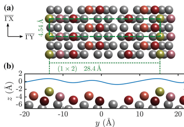
Fig. 1 (a) Top view of the (1 \times 2) reconstructed Bi(114) surface. (b) Side view of the atomic structure of Bi(114) surface along the \Gamma\bar{Y} -direction, illustrating the asymmetry upon scattering normal to the steps. An exemplary corrugation function (eqn (3)) using j = 3 terms with h = [0.435, 0.43, 0.14] and \alpha = \left[-\frac{\pi}{2}, \frac{\pi}{2}, \frac{\pi}{2}\right] is drawn as solid blue line above the side view of the atomic structure.
