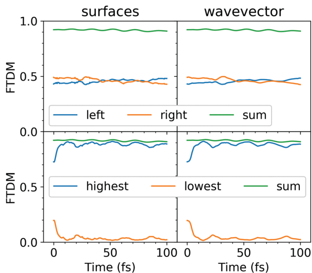
Fig. 3 Ensemble-averaged \text{FTDM}_{LL(RR)}(t) (upper panels) and \text{FTDM}_{\mathcal{H}(L)}(t) (lower panels), calculated using the “surfaces” (left) and “wavevector” (right) methods. The sums \text{FTDM}_{LL}(t) + \text{FTDM}_{RR}(t) (upper panels) and \text{FTDM}_{\mathcal{H}}(t) + \text{FTDM}_{\mathcal{L}}(t) (lower panels) are also shown.
