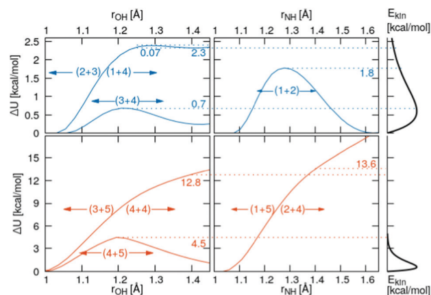
Fig. 6 Top row: Quantum-mechanical scans of the reacting pairs in the simple protonation scheme. Bottom row: Additional reactions in the advanced protonation scheme. The right panel concerns the Maxwell-Boltzmann distribution of the kinetic energy.
