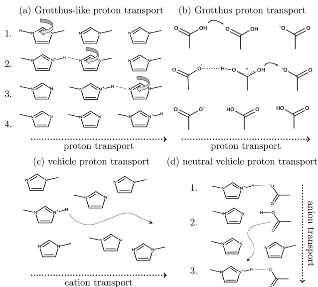
Fig. 2 Various charge transport mechanisms for the conductivity in protic ionic liquids. Grotthus-like proton transport (a) is also possible using a rotating acetic acid molecule. A direct Grotthus-mechanism can be realized via protonated acetic acid molecules (b). Vehicle transport can be realized via cations (c) or neutral acetic acid (d).
