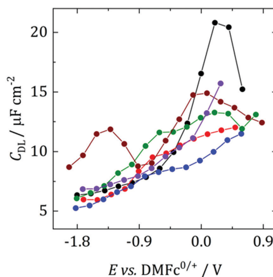
Fig. 2 Differential capacitance curves for 100 mM [ n\text{Bu}_4 ][BF 4 ] at a r = 0.25 mm Pt electrode, scanning in the anodic direction. Black: DCM, red: TFT, blue: o DCB, green: pFT, brown: CB, purple: DCE.
