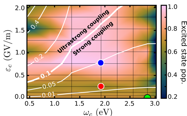
Fig. 3 Population in the excited state, at 400 fs, as a function of the cavity resonance frequency \omega_c and field strength \varepsilon_c . The coupling strength ( g_{ij}/\omega_c ) is shown by the contour lines. The colored dots mark the position of the cases considered in Fig. 4 and in the discussion.
