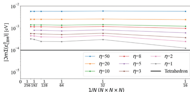
Fig. 4 Convergence of \Im m\Sigma_{\text{CBM}}(\epsilon_{\text{CBM}}^0) using the DM approach with N , for different values of \eta , at 300 K. Exactly at the CBM, the standard method converges slowly down to the tetrahedron value, as the value of \Sigma is very small and comparable to the “infinitesimal” \eta itself. The tetrahedron value is calculated with N = 160 . The y-axis is in logarithmic scale.
