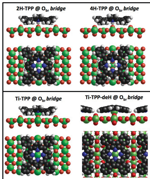
Fig. 18 Top: Side and top views of the equilibrium configurations for isolated 2H- and 4H-TPP molecules (left and right, respectively) on the r-TiO 2 (110) surface. Bottom: Equilibrium configurations of an isolated TiO 2 br -TPP molecule (left) and a flat TiO 2 br -TPP-deH species in its (2 × 6)-rect phase (right).
