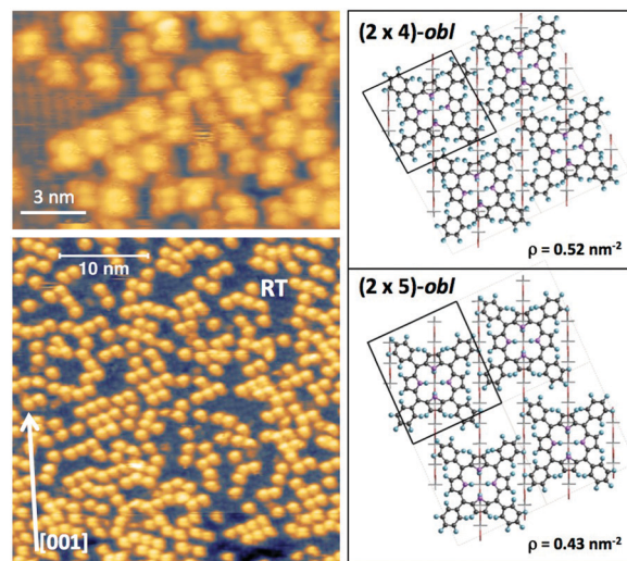
Fig. 12 Left: STM images (Colibri tip) of a \sim 0.5 ML film of 2H-TTP deposited at RT, where small domains with local (2 × 4)-obl order start to form; top and bottom panels correspond to the same film measured at positive (+1.3V, 40 pA) and negative (−1.3 V, 140 pA) biases, respectively. Right: Top views of the (2 × 4)-obl and (2 × 5)-obl phases are shown in the top and bottom panels, respectively.
