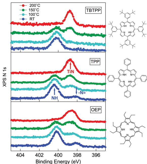
Fig. 10 From top to bottom: the N 1s spectra of 2H-TBTTP (0.8 ML), 2H-TTP (1.1 ML) and 2H-OEP (1.1 ML) as deposited at RT and after annealing; the annealing temperatures are indicated in the top panel; arrows in the central panel (TPP) mark the binding energies of pyrrolic (NH), iminic (=N-) and metalated (TiN) nitrogen. Reproduced from ref. 48 with permission from Elsevier, Copyright 2021.
