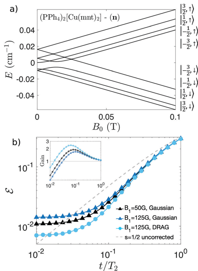
Fig. 4 (a) Energy levels of (PPh 4 ) 2 [Cu(mnt) 2 ] n, consisting of a \text{Cu}^{2+} ion (electronic spin s^A = 1/2 ), coupled to the nuclear I = 3/2 spin by hyperfine interaction (as reported in ref. 28), as function of the external field B_0 . The composition of the eigenstates is indicated on the right. (b) Symbols: error after implementation of the QEC scheme with T_2 = 0.5 ms, B_0 = 0.1 T, T_2^A = 68 \mu\text{s} (as reported in ref. 28), B_1^Q = 30 G, with different forms of the driving fields B_1^Q : Gaussian (triangles) and DRAG (circles). Dashed grey line: error for an uncorrected s = 1/2 spin due to decoherence. Inset: Corresponding gain, i.e. ratio between errors on an uncorrected qubit and on a protected system.
