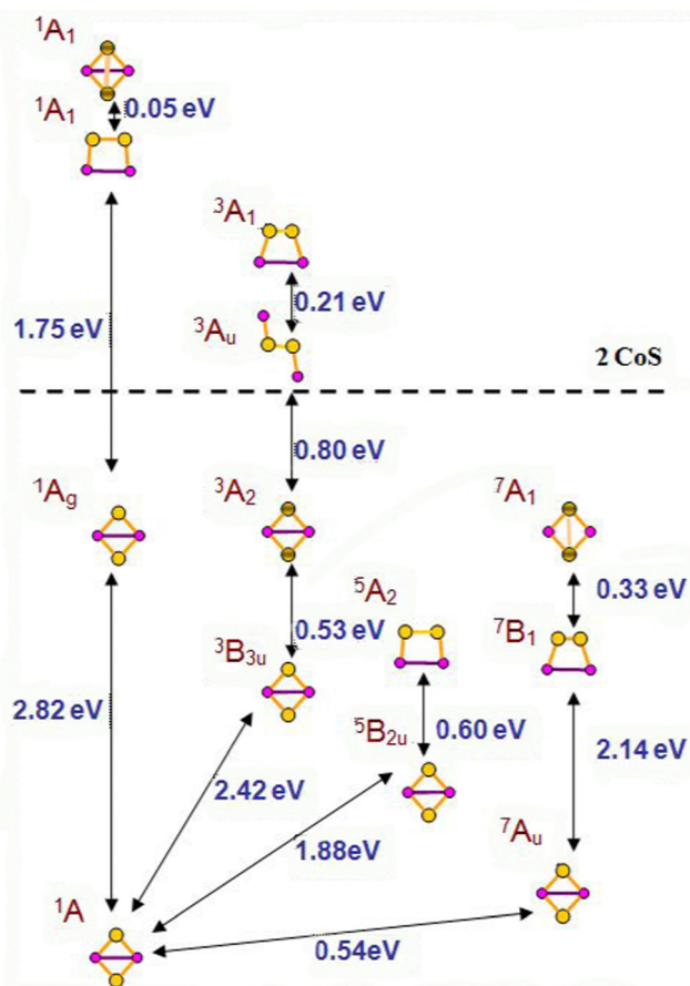
Fig. 3 The global minimum ^1A , corresponding to the antiferromagnetic planar rhombic \text{Co}_2\text{S}_2 , and isomers in higher multiplicity channels: triplets, quintets and septets. The dissociation limit to \text{CoS} is denoted. Co atoms are small red circles, S atoms – yellow large circles; shaded circles denote atoms shifted above the molecular plane in non-planar geometry. The arrows denote the energy difference \Delta E_{\text{tot}} , corresponding to adiabatic transitions, with zero-point and dispersion corrections included.
