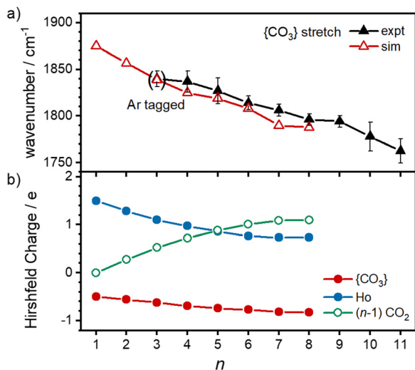
Fig. 8 (a) Observed and calculated wavenumber of the C=O stretch in the \{\text{CO}_3\} moiety of C-isomers as a function of complex size. Uncertainties represent the half-width at half maximum of the experimental peaks. (b) Trends in the Hirshfeld charges on the \{\text{CO}_3\} moiety (red), Ho atom (blue, solid) and the \text{CO}_2 ligands (green, open circles) with increasing complex size.
