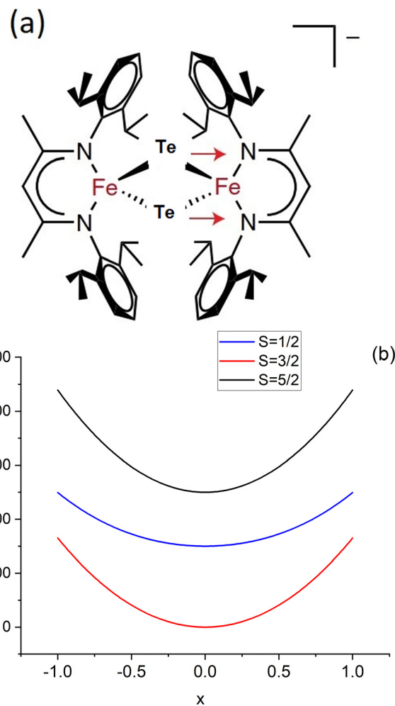
Fig. 4 (a) Representation of the anion [\text{L}_2\text{Fe}_2\text{Te}_2]^- , the red arrows depict the asymmetric (symmetry breaking) mode ( q ); (b) adiabatic ground state ( S = 3/2 ) and two lowest ( S = 1/2 , S = 5/2 ) excited states along q ; The curves were plotted taking the values of J = -200 \text{ cm}^{-1} and B = 750 \text{ cm}^{-1} (from ref. 10) and the vibronic coupling energy \lambda = 480 \text{ cm}^{-1} (see Table 7).
