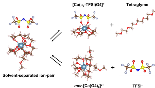
Fig. 2 Molecular representation of the [ mer -[Ca(G4) 2 ] 2 /TFSI] + solvent-separated ion-pair and its evolution to the trans -[Ca(μ 2 -TFSI)(G4)] + contacting ion-pair and free ions.
