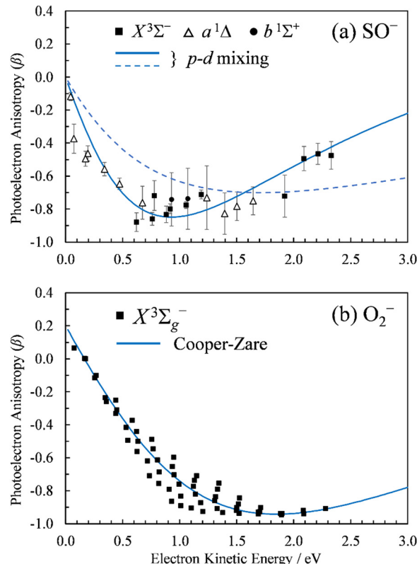
Fig. 2 Photoelectron anisotropy parameter ( \beta ) as a function of eKE for (a) SO - and (b) O 2 - . The SO - data in (a) correspond to the 611 nm (2.03 eV), 532 nm (2.33 eV), and 355 nm (3.49 nm) experimental results presented in Fig. 1. The blue solid curve in (a) is a 2p-3d mixing curve calculated using eqn (2) with \gamma_d = 0.81 , A_1 = 0.53 \text{ eV}^{-1} , A_2 = 0.10 \text{ eV}^{-1} , B_2 = 11.4 \text{ eV}^{-1} , and \cos \delta_{2,0} = \cos \delta_{3,1} = 0.96 . The dashed curve corresponds to A_1 = 0.35 \text{ eV}^{-1} , B_2 = 1.7 \text{ eV}^{-1} , with all other parameters unchanged (see the text for details). The curve in (b) is defined by Hanstorp's implementation of the Cooper-Zare equation [or, equivalently, eqn (2) with \gamma_d = 1 ], using A_2 = 0.36 \text{ eV}^{-1} and \cos \delta_{3,1} = 0.96 .
