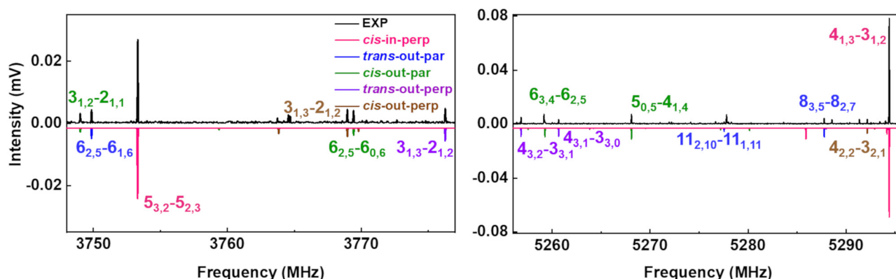
Fig. 3 Parts of the 2–8 GHz rotational spectrum of AMPA with the labelling scheme of the rotational transitions as J'_{K'_a K'_b K'_c} \leftarrow J''_{K''_a K''_b K''_c} . The top part shows the experimental spectrum and the bottom part represents the simulations using the fitted rotational parameters for AMPA conformers (Table 2). The relative intensities are based on the predicted dipole moment components (Table 1).
