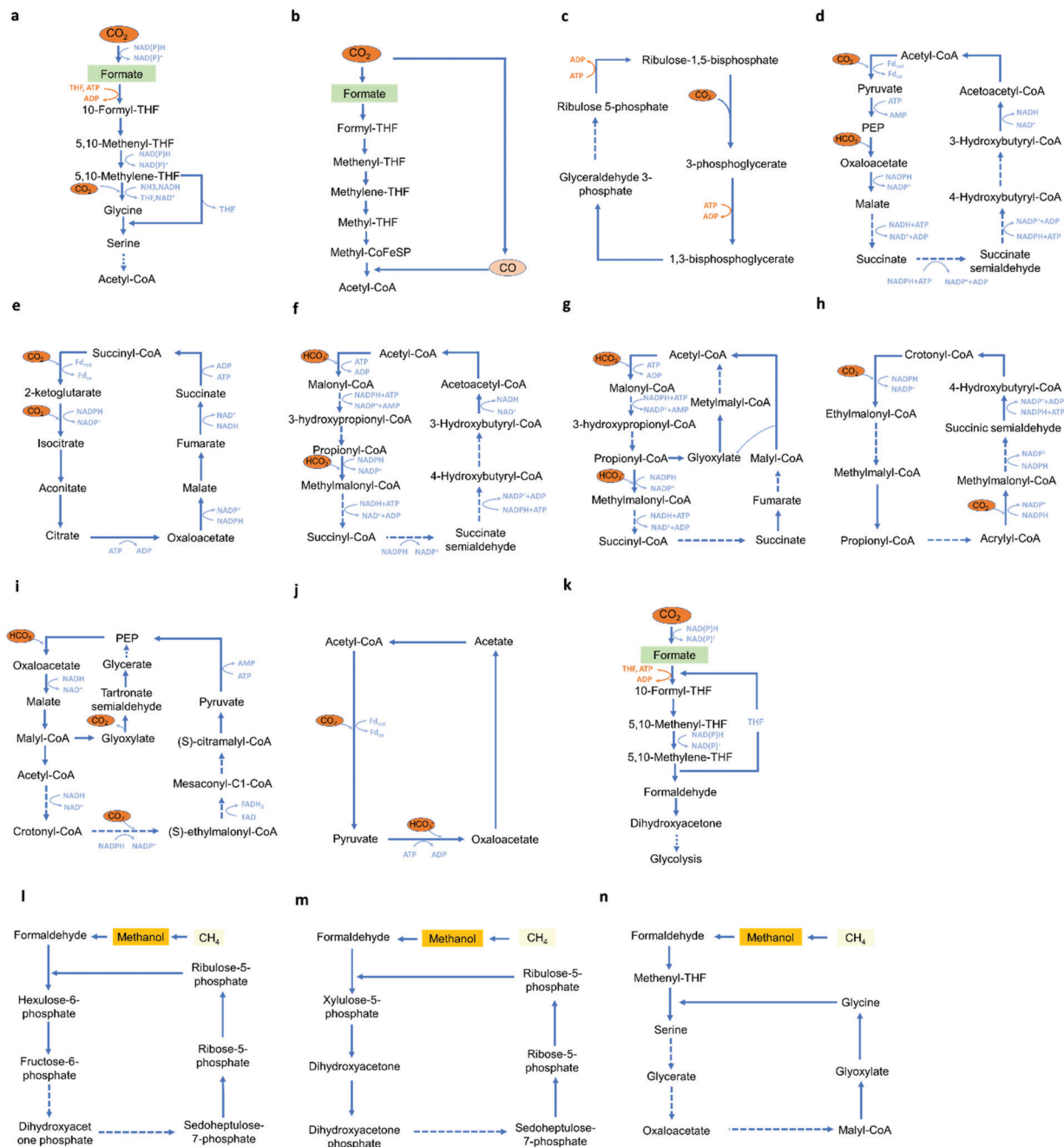
Fig. 8 Representations of current C1 utilization pathways. (a) The reductive glycine pathway. (b) The Wood-Ljungdahl pathway. (c) The CBB cycle. (d) The DC/HB cycle. (e) The reductive TCA cycle. (f) The HP/HB cycle. (g) 3-HP bicycle. (h) The CETCH cycle. (i) The rGPS-MCG cycle. (j) The POAP cycle. (k) The HWLS pathway. (l) The RuMP cycle. (m) The XuMP cycle. (n) The serine cycle.
