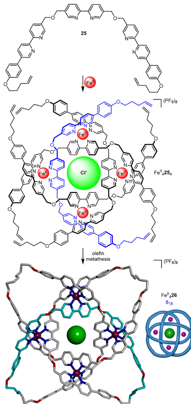
Fig. 9 Synthesis of 8_{19} knot \text{Fe}_6^{II}26 via braiding of three ligand strands. 59
