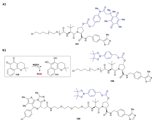
Fig. 47 Enzymatically activated PROTACs. Quinone-caged HaloPROTAC 107 activated by NQO1-mediated reduction (a) and generation of ROS via NQO1-mediated reduction of \beta -lapachone ( 110 ) activating ROS-responsive HaloPROTAC 108 and BET degrader 109 (b). 194
