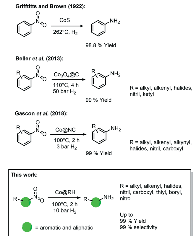
Scheme 1 Historical development of cobalt-catalyzed synthesis of amines by hydrogenation of nitro compounds.
