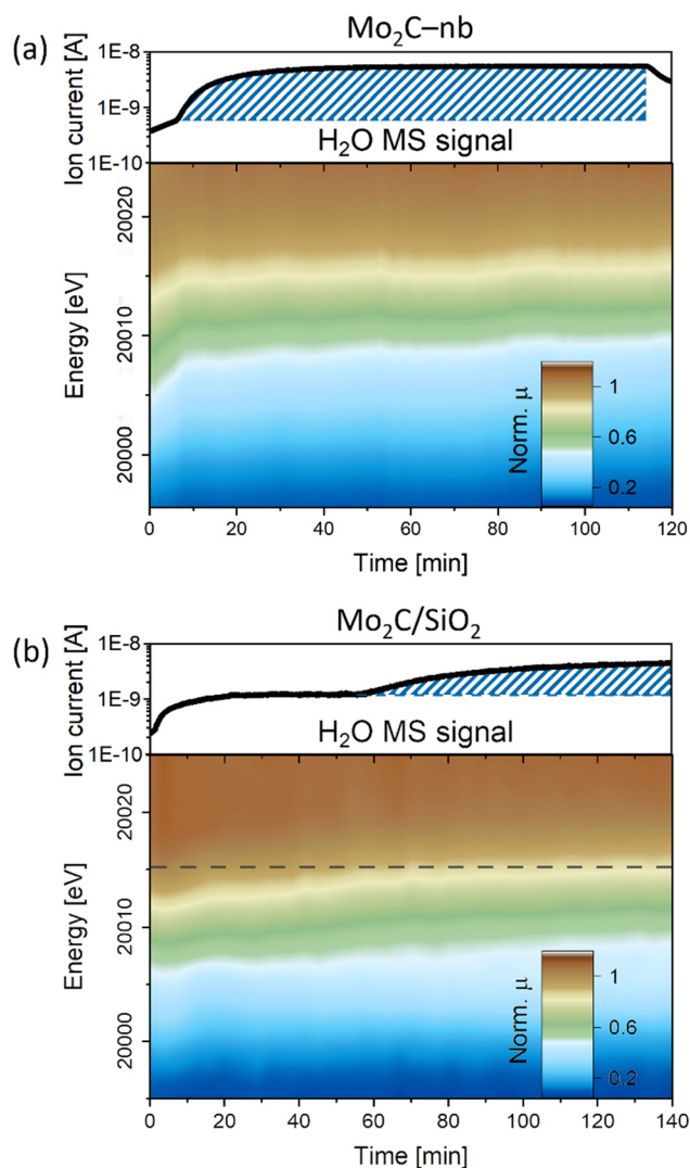
Fig. 3 In situ Mo K-edge XANES (contour plots of the intensity as a function of energy and time) during DRM (capillary reactor, 730 °C, 8 bar) of a) Mo 2 C-nb ( W/F = 45 \text{ ms g}_{\text{Mo}} \text{ mL}^{-1} ) and b) Mo 2 C/SiO 2 ( W/F = 0.8 \text{ ms g}_{\text{Mo}} \text{ mL}^{-1} ), complemented by the evolution of H 2 O MS signal.
