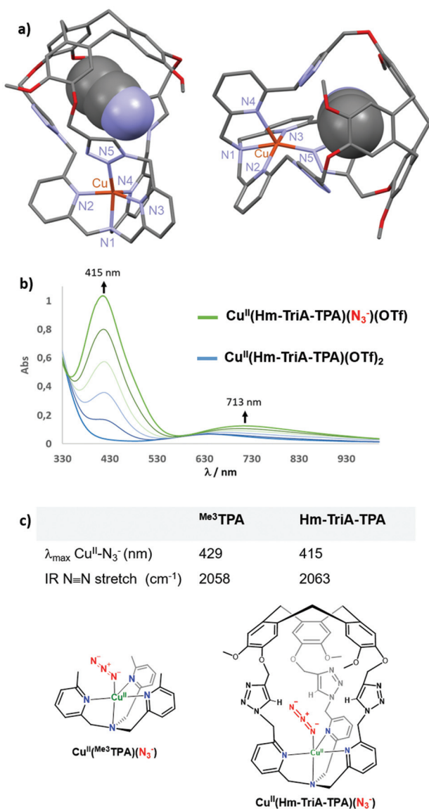
Fig. 3 (a) Views of the X-ray crystal structure of Cu II (Hm-TriA-TPA)(OTf) 2 . (b) UV-vis monitoring of the formation of the azido adduct Cu II (Hm-TriA-TPA)(N 3 )(OTf) upon addition of NBu 4 N 3 (0 to 1.0 equiv.) to a 0.5 mM solution of Cu II (Hm-TriA-TPA)(OTf) 2 in acetone. (c) Spectroscopic features (UV-vis and IR) of the azido complexes stabilized by Me 3 -TPA and Hm-TriA-TPA.
