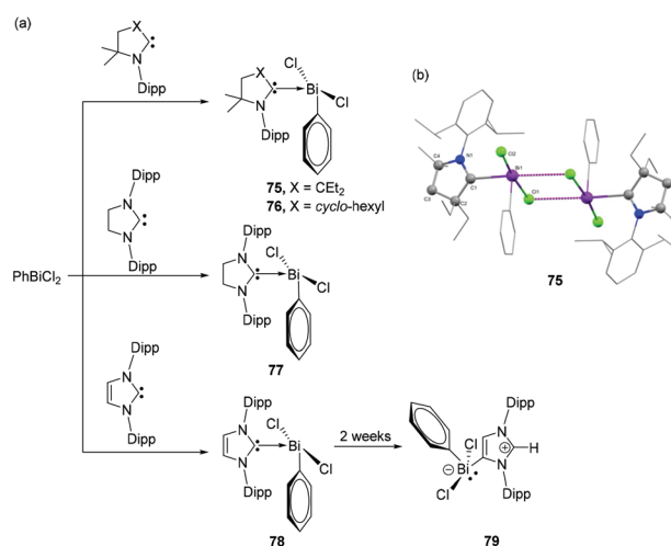
Fig. 25 (a) Syntheses of CAAC-stabilized bismuth adducts 75 – 79 ; solid-state structure of 75 .
