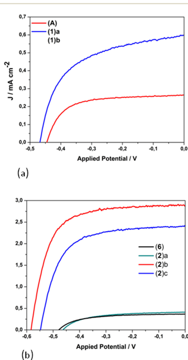
Fig. 13 J – V curves for the copper(I)-based dyes 1, [Cu(pqcame 2 )]PF 6 (A) (a); 2 and 6 (b). Lower case letters highlight the different architecture of the semiconductor material of the anode, dyed with 1 and 2, as reported in Table 2.
