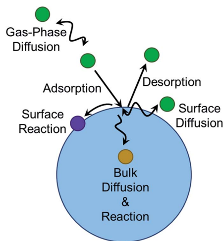
Fig. 10 Multiphase reaction pathways. Molecules diffusing in the gas phase that encounter an aerosol particle may adsorb to the surface, diffuse within the surface region, react within the surface region, diffuse into the bulk, and react in the bulk. The impinging gas-phase molecule can also desorb without reacting, and products can remain at the surface, remain in the bulk, or desorb into the gas phase.
