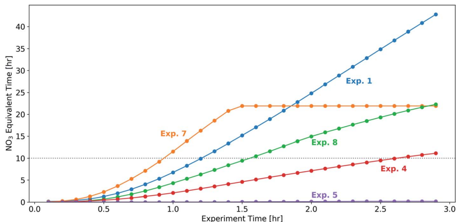
Fig. 7 The equivalent number of hours in an ambient urban environment (assuming an NO 3 radical concentration 20 ppt throughout the night) for the subset of experiments with NO 3 radical measurements.
