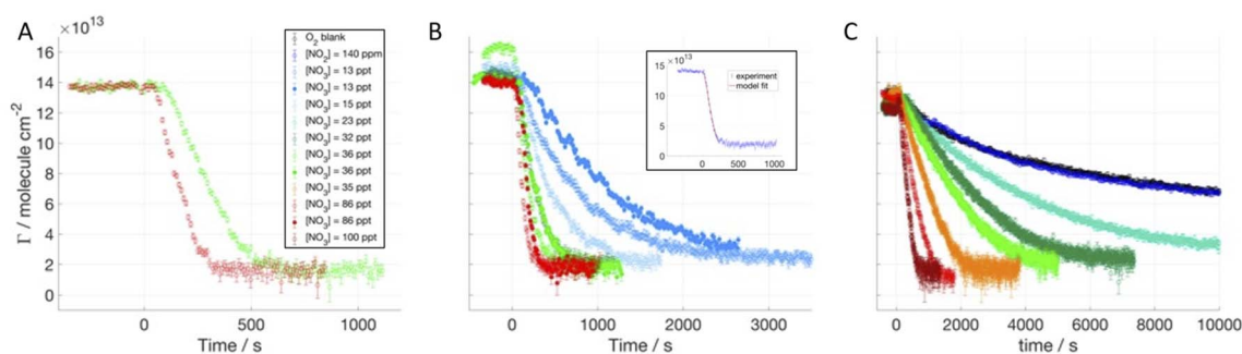
Fig. 4 Surface excess decays of d\text{MOhMO} (A), d\text{MOhSA} (B), and d\text{MOhOA} (C) exposed to different [\text{NO}_3] ; mean values of \text{NO}_3 mixing ratios are displayed in the legend (1 ppt = 2.7 \times 10^7 molecule per \text{cm}^3 ), \text{NO}_3 is admitted at t = 0 \text{ s} . In the insert, data and fit are shown for d\text{MOhSA} exposed to [\text{NO}_3] = 86 \text{ ppt} .
