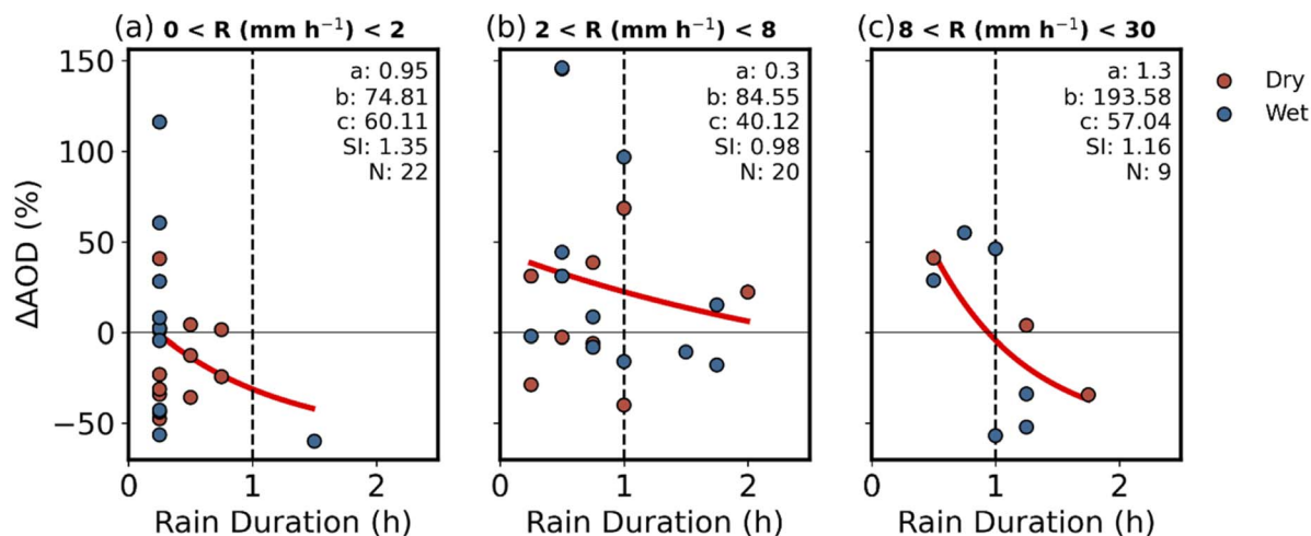
Fig. 4 Scatterplots of the percent difference in AOD post-rain event ( \Delta AOD; %) as a function of rain duration (hours) and colored by season. Data are stratified by rain rate ( R ; \text{mm h}^{-1} ): (a) 0 < R < 2 , (b) 2 < R < 8 , (c) 8 < R < 30 . Wet (dry) season is defined as May to October (November to April). Number of data points per panel ( N ) is provided. The black dashed vertical lines mark the median rain duration based on Fig. 3c. Curve-fitting was performed as in Fig. 3a (see Section 2.4).
