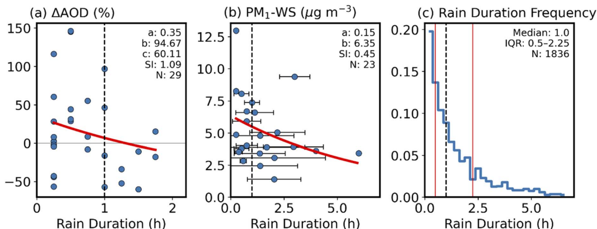
Fig. 3 Scatterplots of the (a) percent difference in AOD before and after rain events ( \Delta AOD; %; 2012–2019). (b) MOUDI total water-soluble species ( \text{PM}_1 -WS; \mu\text{g m}^{-3} ; 2018–2019) as a function of rain duration (hours). (c) Histogram of rain duration (2010–2020). Rain duration in (b) refers to the mean duration of all rain events during each MOUDI set with error bars along the x-axis representing one standard deviation. Note that points in (b) without error bars consist of single rain events. The black dashed vertical lines in (a–c) mark the median rain duration based on (c). In (c), the red lines represent the 25th–75th percentile range (interquartile range, IQR). Number of data points per panel ( N ) is provided. Only data from the wet season were plotted (May–October). Curve-fitting for (a and b) is described in Section 2.4.
