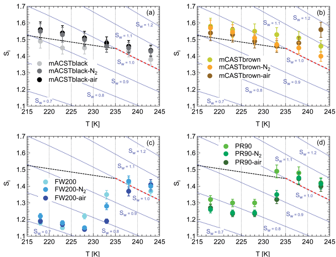
Fig. 2 Onset (at \text{AF} = 0.1\% ) ice saturation ratio ( S_i ) as a function of T for fresh and denuded 400 nm mCASTblack (a), mCASTbrown (b), FW200 (c) and PR90 (d). \text{AF} is reported from the 1.0 \mu\text{m} OPC channel. Black dashed line: homogeneous freezing conditions for solution droplets at T < \text{HNT} , according to Koop et al. 45 Light blue dotted line: constant water saturation conditions calculated based on Murphy and Koop. 44 Red dashed line: the 1.0 \mu\text{m} size water droplet survival conditions for T > \text{HNT} , where the phase of the particle larger than 1.0 \mu\text{m} can be either ice or liquid water. The S_i uncertainty due to the temperature uncertainty ( \pm 0.1 K) of the HINC chamber is indicated as error bars. Each data point was derived from the \text{AF} curves in Fig. 9–12 presented in the Appendix in which each \text{AF} curve is an average of at least two individual RH ramps.
