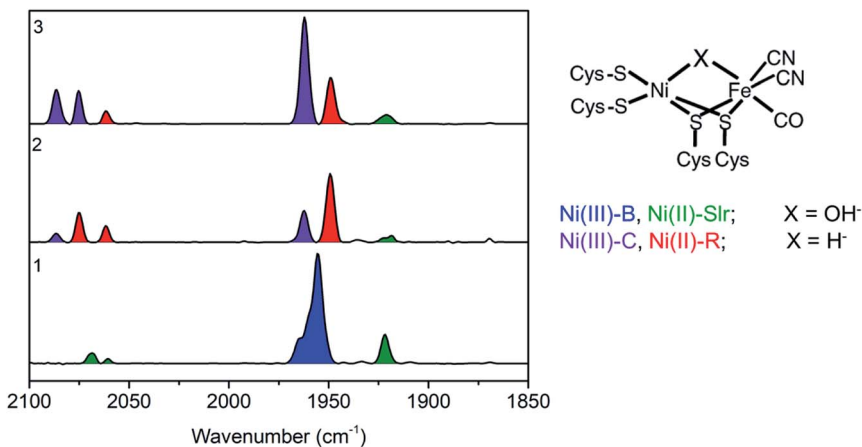
Fig. 2 (Left) Baseline corrected FTIR spectra of a DvMF [NiFe] hydrogenase as isolated 1, incubated 4 hours in H 2 atmosphere 2, and in 15 µl of viologen and 40 µl NaDT 3. Band positions for the different state are as follows: Ni(III)-B (1955, 2081, and 2090 cm -1 ), Ni(II)-Sl r (1922, 2061, 2070 cm -1 ), Ni(III)-C (1961, 2074, 2085 cm -1 ), Ni(II)-R (1948, 2061, 2074 cm -1 ). (Right) Schematic representation of DvMF [NiFe] hydrogenase active site, where X is identified for each redox state.
