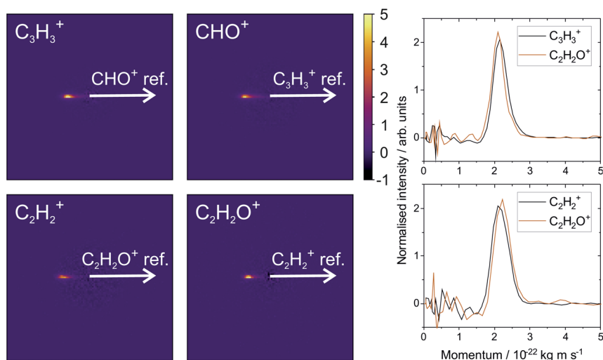
Fig. 2 Recoil-frame covariance images obtained following electron ionisation of furan at an electron energy of 100 eV, between \text{C}_3\text{H}_3^+ and \text{HCO}^+ , and \text{C}_2\text{H}_2^+ and \text{C}_2\text{H}_2\text{O}^+ . All covariance maps show the characteristic form of a two-body dissociation. The corresponding momentum distributions given on the right show that momentum is conserved as expected.
