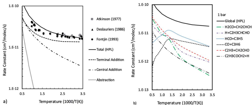
Fig. 4 Total rate constants for the \text{O}(\text{}^3\text{P}) + 1,3\text{-butadiene} reaction compared with experimental data 48,50,51 and contributions of addition to central and terminal carbon atoms and abstraction (a), and channel specific rate constants computed as a function of temperature at 1 bar (b).
