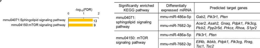
Fig. 5 The effects of soy isoflavone on the functional enrichment analysis of predicted target genes of differentially expressed microRNAs (DEMs). (A) Significant KEGG pathways of predicted target genes of 10 mature DEMs (left) in the red section (HF vs. CON) and 7 mature DEMs (right) in the gray section (HF/S vs. CON only). In the case of the HF vs. CON comparison, top 20 significant pathways are depicted. The pathways colored in blue represent the pathways identified only in the gray section of the Venn diagram. (B) Significant KEGG pathways of predicted target genes of DEMs from the 'HF/SI vs. HF/S' comparison. DEMs and the predicted target genes contributing to each significant pathway are indicated in the table. KEGG pathways are indicated in ascending order of FDR. The number of target genes included in each pathway is depicted on the right side of each bar. CON, the group fed with a control diet; HF, the group fed a high-fat diet; HF/S, the group fed with a high-fat/low-isoflavone soy protein diet; and HF/SI, the group fed with a high-fat/high-isoflavone soy protein diet.
