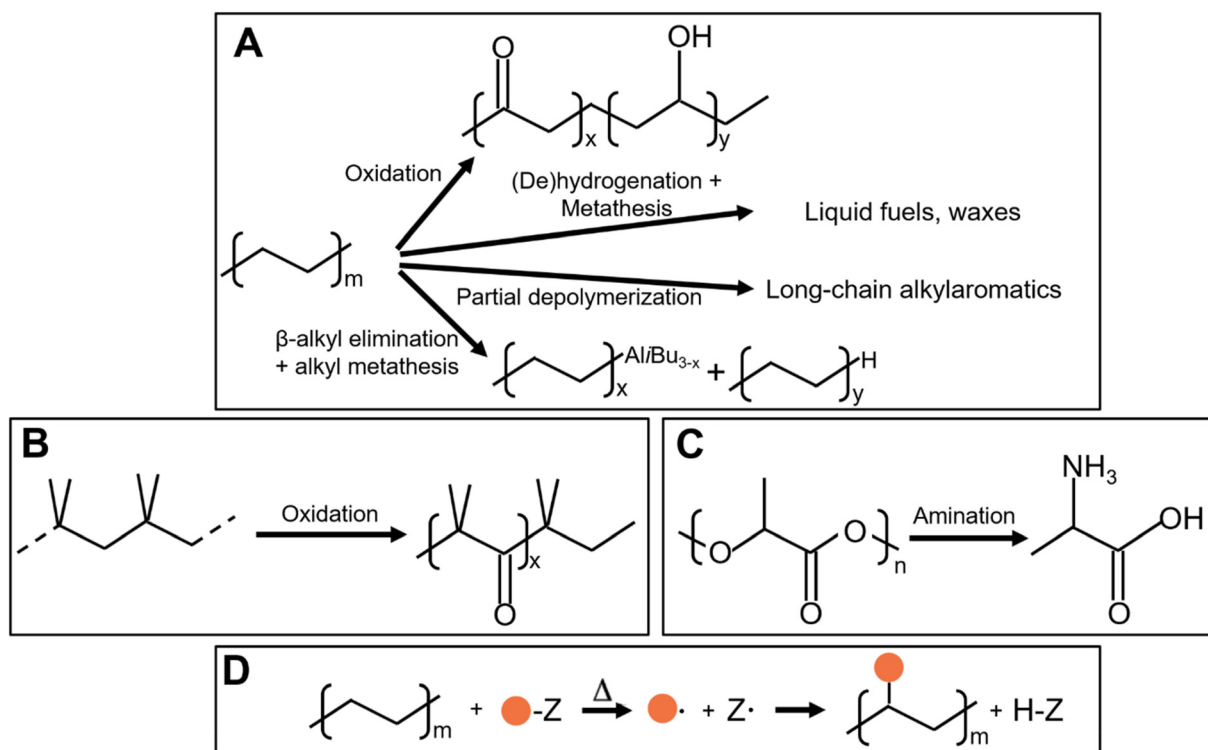
Fig. 41 Strategies in functionalization of plastics: (A) functionalization of polyolefins; (B) oxidation of polyisobutene; (C) PLA amination; (D) reactive extrusion where orange circle represents a function group.
