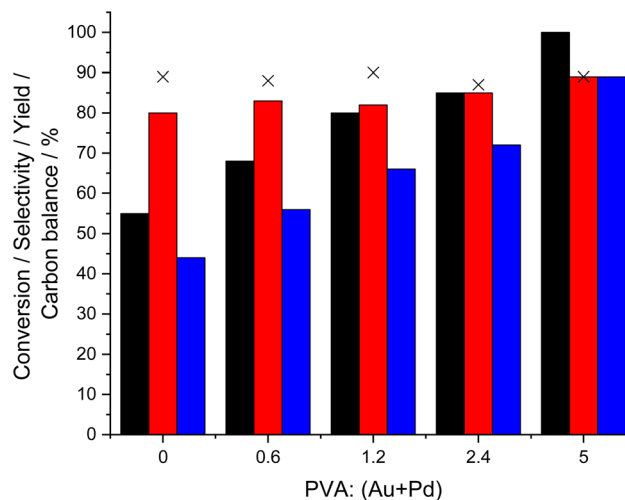
Fig. 3 Effect of PVA: metal ratio on catalytic activity of the 0.33% Au–0.33% Pd/TS-1 catalyst activity towards the ammoximation of cyclohexanone oxime via in situ H 2 O 2 synthesis. Ammoximation reaction conditions: cyclohexanone (2 mmol), NH 4 HCO 3 (4 mmol), 5% H 2 /N 2 (420 psi), 25% O 2 /N 2 (160 psi), catalyst (0.075 g), t -BuOH (5.9 g), H 2 O (7.5 g), 3 h, 80 °C 800 rpm. Key: cyclohexanone conversion (black bar), selectivity towards oxime (red bar), cyclohexanone oxime yield (blue bar), carbon balance (crosses). Note: all catalysts were exposed to an oxidative heat treatment prior to use (static air, 400 °C, 3 h).
