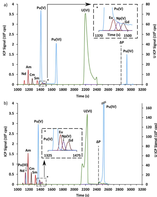
Fig. 4 (a) Electropherogram obtained by CE-Q-ICP-MS for a spent MOX fuel sample with a 120 \text{ mmol L}^{-1} \alpha -HMBA electrolyte one day after the end of the oxidation step. (b) Electropherogram obtained by CE-Q-ICP-MS for a spent MOX fuel sample with a 120 \text{ mmol L}^{-1} \alpha -HMBA electrolyte seven days after the end of the oxidation step. For both electropherograms, it was necessary to apply 1 bar of pressure in order for Pu(IV) to migrate. The time at which the pressure ( \Delta P ) was applied is symbolized as a dashed line.
