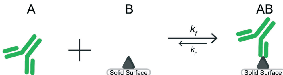
Scheme 1 Reaction between species A and species B to form species AB.
