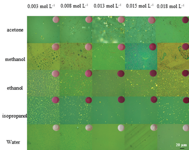
Fig. 1 OM images of nanocomposites with a 100× magnification. Vertical direction including acetone, methanol, ethanol, isopropanol, and water samples, horizontal direction where the TCA solution ranges from 0.003 to 0.018 mol L -1 . Inset: Images obtained using a digital camera of 25 samples. Scale bar: 20 μm.
