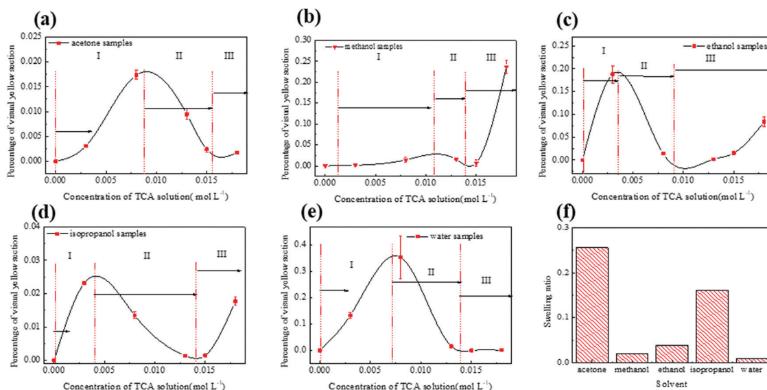
Fig. 2 Percentage of the visual yellow section to the surface area of Au-free PDMS solvent samples and the swelling ratio of each solvent: (a) acetone, (b) methanol, (c) ethanol, (d) isopropanol, and (e) water. (f) The swelling ratio of the solvent to the PDMS matrix.
