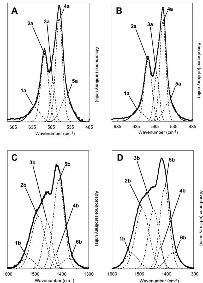
Fig. 5 Deconvolution of the (A and B) OH L and PO 4 ν 4 and (C and D) CO 3 ν 3 regions of the FTIR spectra of the as-prepared x = 1.5 compositions for (A and C) Series I (K 2 CO 3 ) and (B and D) Series II (KHCO 3 ) potassium-carbonate co-substituted samples showing the various vibrations that contribute to the observed spectra; y-axis is an arbitrary scale. Dashed lines correspond to the individual fitted peaks and the solid line is the corresponding model spectra, with the raw data presented as isolated data points.
