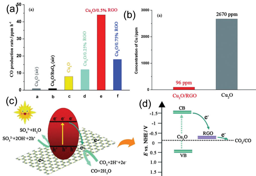
Fig. 13 (a) CO yields over various photocatalysts, (b) plot of leaching of Cu caused by photoreduction, and (c) and (d) schematic illustrations of the CO 2 reduction mechanism and charge transfer in the rGO–Cu 2 O composite. 134 Copyright 2014, Wiley.
