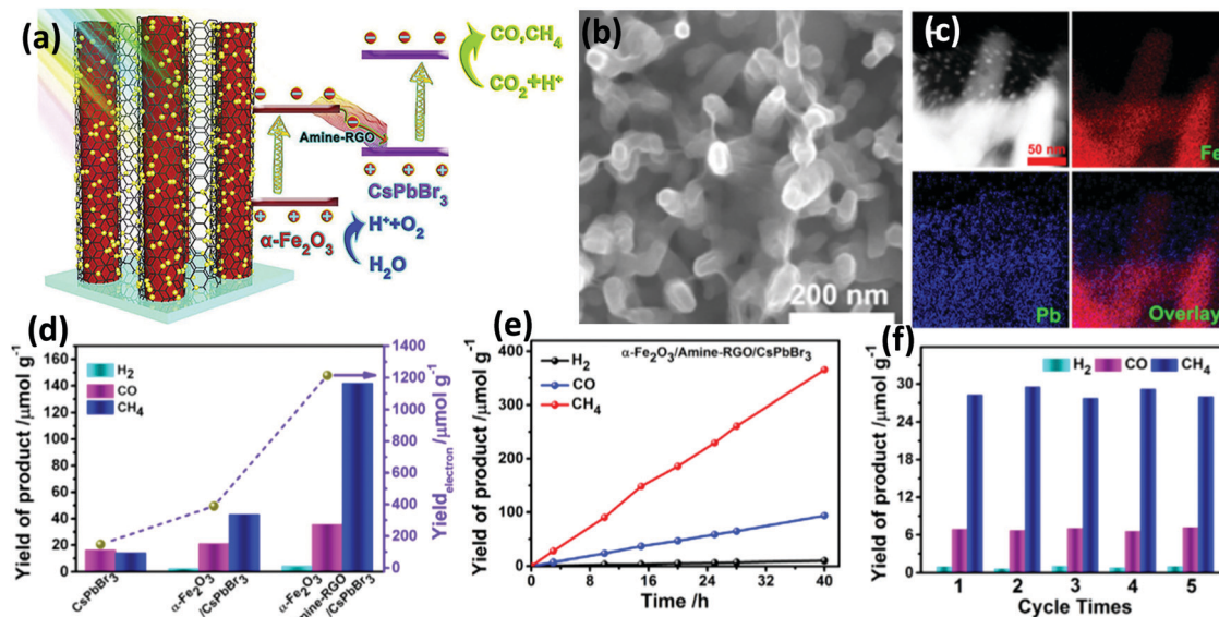
Fig. 18 (a) Schematic illustration of charge transfer and CO 2 photoreduction over the Fe 2 O 3 –amino-rGO–CsPbBr 3 composite, (b) FESEM image, (c) EDS elemental mapping, (d) comparison of CO 2 photoreduction over various photocatalysts, (e) long-term utilization as a photocatalyst and (f) recycling stability tests of Fe 2 O 3 /amine-rGO/CsPbBr 3 . 148 Copyright 2020, Elsevier.
