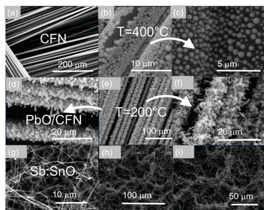
Fig. 6 (a) SEM image of an ordered CFN; (b and c) SEM images of spherical PbO obtained at 400 ^{\circ}\text{C} ; (d–f) one dimensional PbO grown on CFNs at 200 ^{\circ}\text{C} and 10 Pa; (g) SEM image of SnO 2 NWs; (h and i) SEM images of branched SnO 2 /PbO NWs obtained via the growth of PbO over SnO 2 NWs at T = 300 ^{\circ}\text{C} and 10 Pa.
