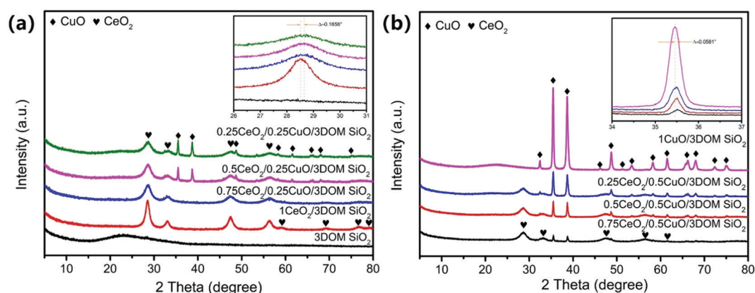
Fig. 3 XRD patterns of CeO 2 /CuO/3DOM SiO 2 series catalysts: (a) loaded with different contents of CeO 2 (inset: amplified patterns in 26\text{--}31^\circ ) and (b) loaded with different contents of CuO (inset: amplified patterns in 34\text{--}37^\circ ).
