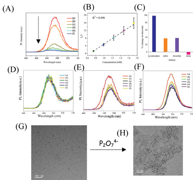
Fig. 3 (A) Emission spectrum of (a) Zn Au NCs and of those following the addition of (b) 15 \mu L, (c) 20 \mu L, (d) 25 \mu L, (e) 30 \mu L and (f) 35 \mu L of 100 mM of sodium pyrophosphate. (B) Corresponding Stern Volmer plot. (C) Bar diagram showing the percentage decrease in the luminescence intensity of Zn Au NCs upon the addition of pyrophosphate and various other interfering agents. (D) Emission spectrum of (a) Zn Au NCs and of those following the addition of (b) 20 \mu L, (c) 30 \mu L, (d) 40 \mu L, (e) 50 \mu L and (f) 60 \mu L of 100 mM of sodium nitrate. (E) Emission spectrum of (a) Zn Au NCs and of those following the addition of (b) 20 \mu L, (c) 30 \mu L, (d) 40 \mu L, (e) 50 \mu L and (f) 60 \mu L of 100 mM of sodium sulphate. (F) Emission spectrum of (a) Zn Au NCs and of those following the addition of (b) 20 \mu L, (c) 30 \mu L, (d) 40 \mu L, (e) 50 \mu L and (f) 60 \mu L of 100 mM of sodium thiosulphate. (G) Transmission electron microscopic image of Zn Au NCs and (H) of that following the addition of 30 \mu L of 100 mM sodium pyrophosphate.
